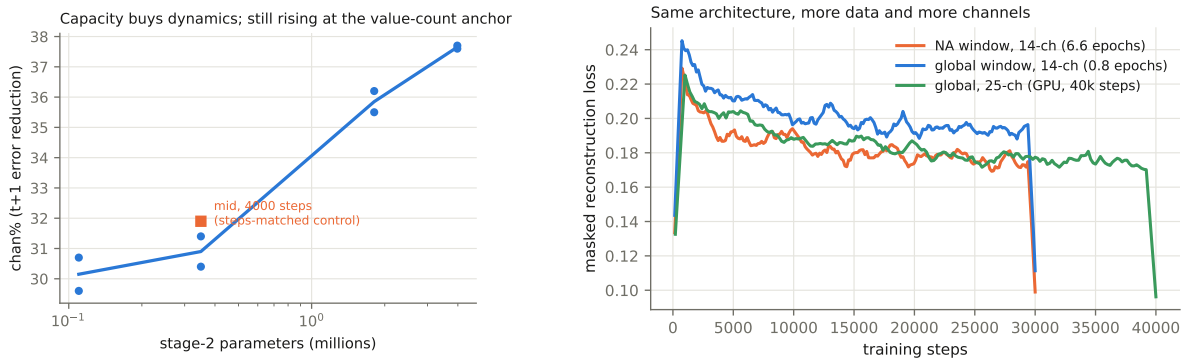
Figure 14: Left: the original stage-2 capacity sweep (0.11–4M parameters, 12-channel coarse tensor, no stencil) — the first sign, in retrospect, that stage-2 capacity was the binding axis; it was still rising at its top end. Right: codec training curves across generations.
