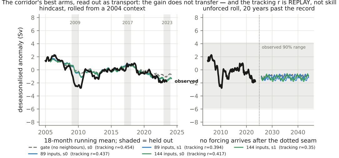
Figure 10: The AMOC read-out of the two widest 205M arms, rolled. Left: hindcast from a 2004 context, with the three never-trained years shaded — those columns were described in v6 as “the honest test, because outside them the roll replays months the codec saw in pretraining”. They are not a test at all, and the legend’s r is not a skill number : §9.2 rolls these same heads from six context ends spanning a decade and finds the tracking correlation flat in lead time and the post-record peaks pinned to fixed calendar months whatever the starting state. The whole left panel — shaded columns included — is trajectory replay, and its r is relabelled here as replay tracking: it measures how completely the head has memorized the record, not how well it forecasts. Right: twenty years of unforced roll past the end of the record. The flatness on the right is the finding, not a forecast: with no wind or heat-flux forcing after the seam, the learned dynamics relaxes toward climatology and stops moving, which is a damped attractor rather than a quiet ocean — and §9.2 adds that what residual motion there is repeats on an integer number of years. Interactive version, with the per-arm table, at blauwelt.github.io/earth/ml/paper/figs/amoc_roll.html .
