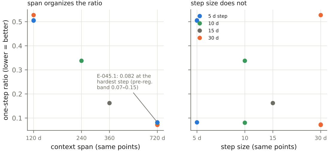
Figure 12: The step \times span factorial. Every measured arm of E-044b/E-045, plotted twice: against context span (left) and against step size (right). Same points, same colors (step size). Span collapses the ratios onto one monotone family; step size scatters them. The decisive rung (E-045.1: 5-day steps at the full 720-day span) landed at 0.082, inside its pre-registered 0.07–0.15 band.
