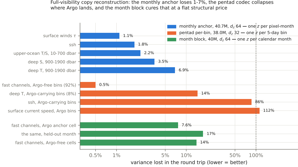
Figure 13: What each codec’s round trip loses , at full visibility — encode and decode with nothing masked and nothing forecast, so this is the representation tax alone. Bars are fraction of channel variance lost ( \text{rmse}^2 in standardized units); the dotted line at 100% is the channel’s own variance, so a bar reaching it carries none of that channel and a constant would have done as well. The monthly anchor is orderly and loses most where the transport integral weights most (deep temperature, 6.9%). The per-bin pentad codec is near-perfect on the 92% of bins that carry no Argo and collapses on the 8% that do — 40 channels competing for 32 latent dimensions. The month-block codec cures that collapse at the anchor and pays a flat structural price everywhere else: one embedding per month is a genuine \approx 4:1 squeeze in time.
