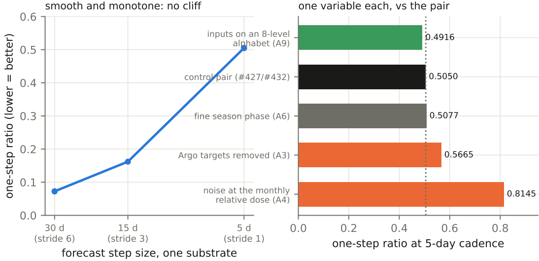
Figure 11: Left: the cadence ladder. One-step forecast ratio against step size, holding everything else fixed — same frozen pentad codec, same embeddings, same 1024 \times 16 head with input noise, same pixels, 20,000 steps, each arm scored against its own persistence baseline. The two points at 30 days are the Argo-carrying and Argo-free bin selections. Smooth and monotone — but K=24 is fixed, so context span co-varies with the step, and §10.3 shows the span is what this curve is measuring. Right: the component ladder at 5 days, one variable per arm against the two-seed control (dotted). Rescaling the exposure-bias noise to the pentad embedding scale is catastrophic, removing the Argo targets makes training worse , a continuous season phase changes nothing, and only restricting the head’s inputs to an 8-level-per-dimension alphabet beats the control. Every arm is n=1 except the control, so these are directions; the control pair’s own |\Delta| is 0.0011.
