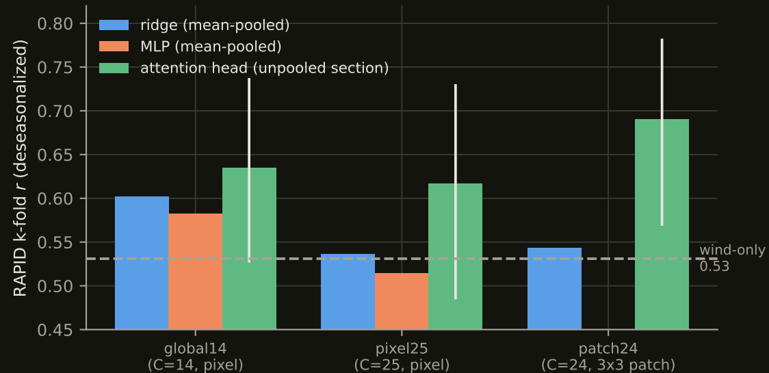
Same frozen embeddings, three read-outs: nonlinearity adds nothing, section structure adds everything
