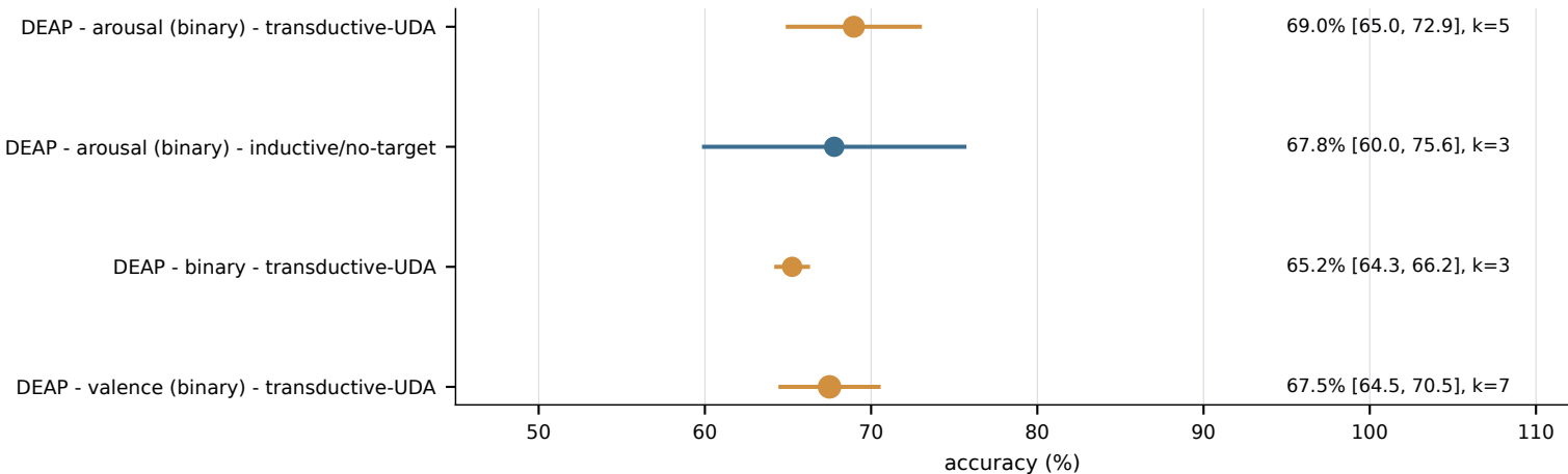
DEAP pooled strata
