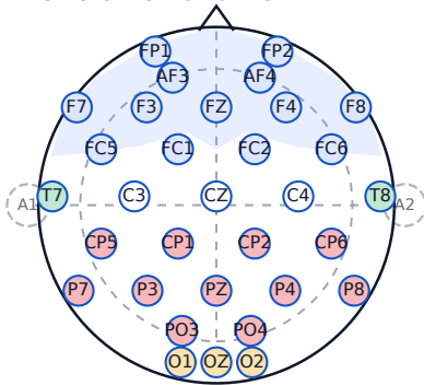
B 32-channel 10-20-like
