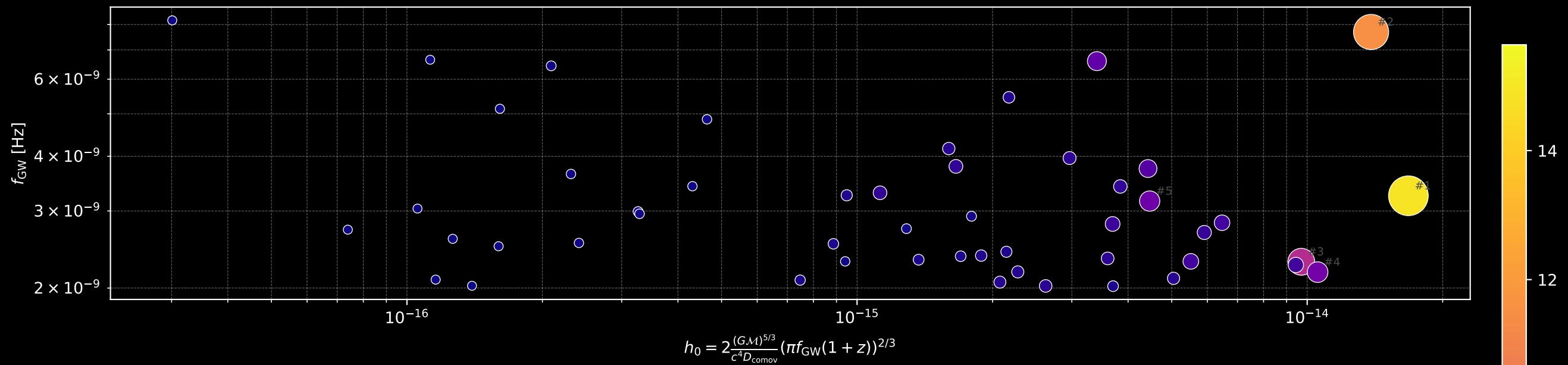
CGW candidate properties — optimal SNR
