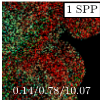
Path tracing
