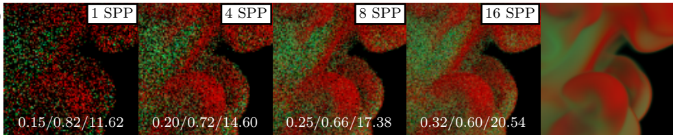
Path tracing
