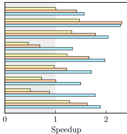
Global illumination
