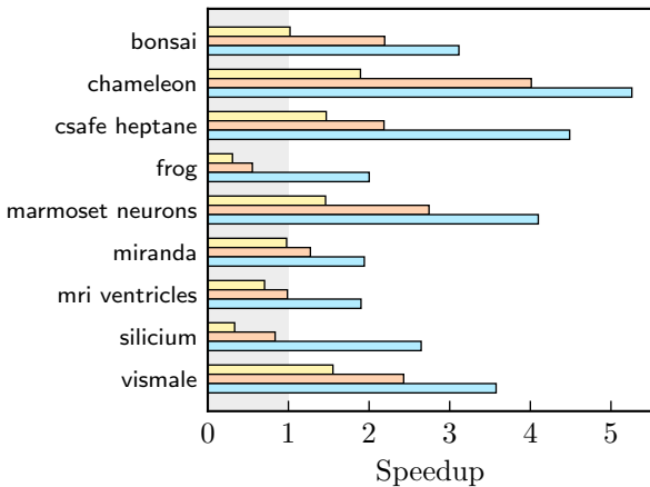
Indirect illumination
