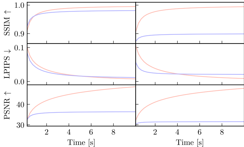
Global illumination
