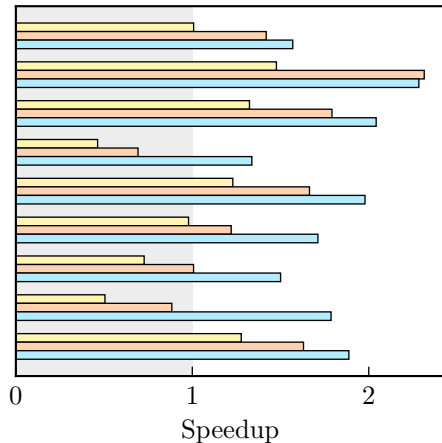
Global illumination
