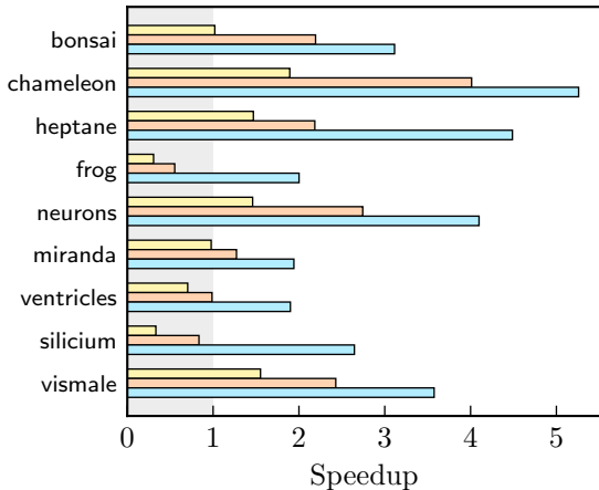
Indirect illumination
