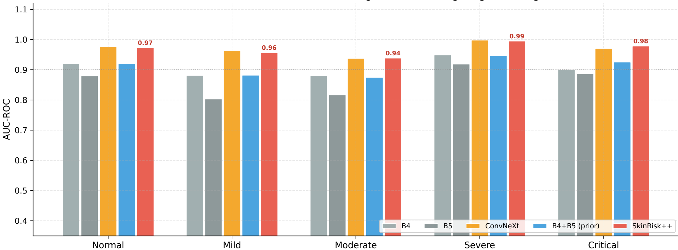
Per-class AUC-ROC across all five configurations — Stage 2 gain is largest
