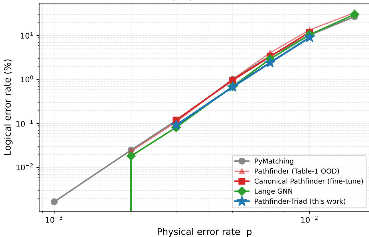
d=7 decoder comparison at matched 4-parameter circuit-level noise (60K shots per point, 95% Wilson CIs)
