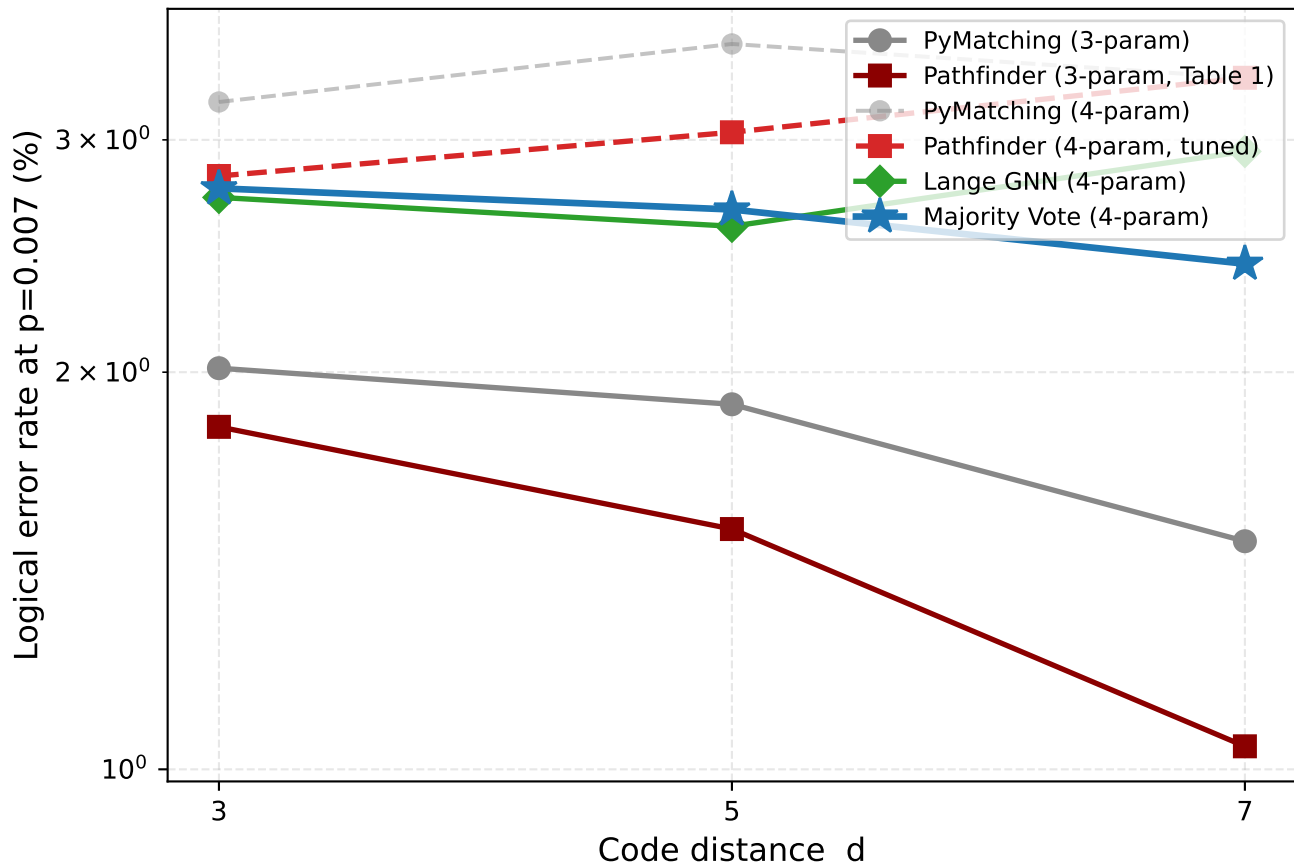
Error-suppression scaling with code distance
