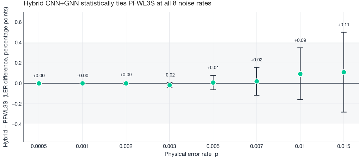
All 8 differences contain zero (error bars cross the zero line). The architectural fusion does not measurably help at this scale.
