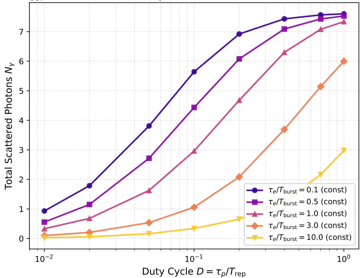
Absolute Yield ( N_p = 10 , E_{\text{tot}} = 1.0\text{J} , z_R = 3534\mu\text{m} )
