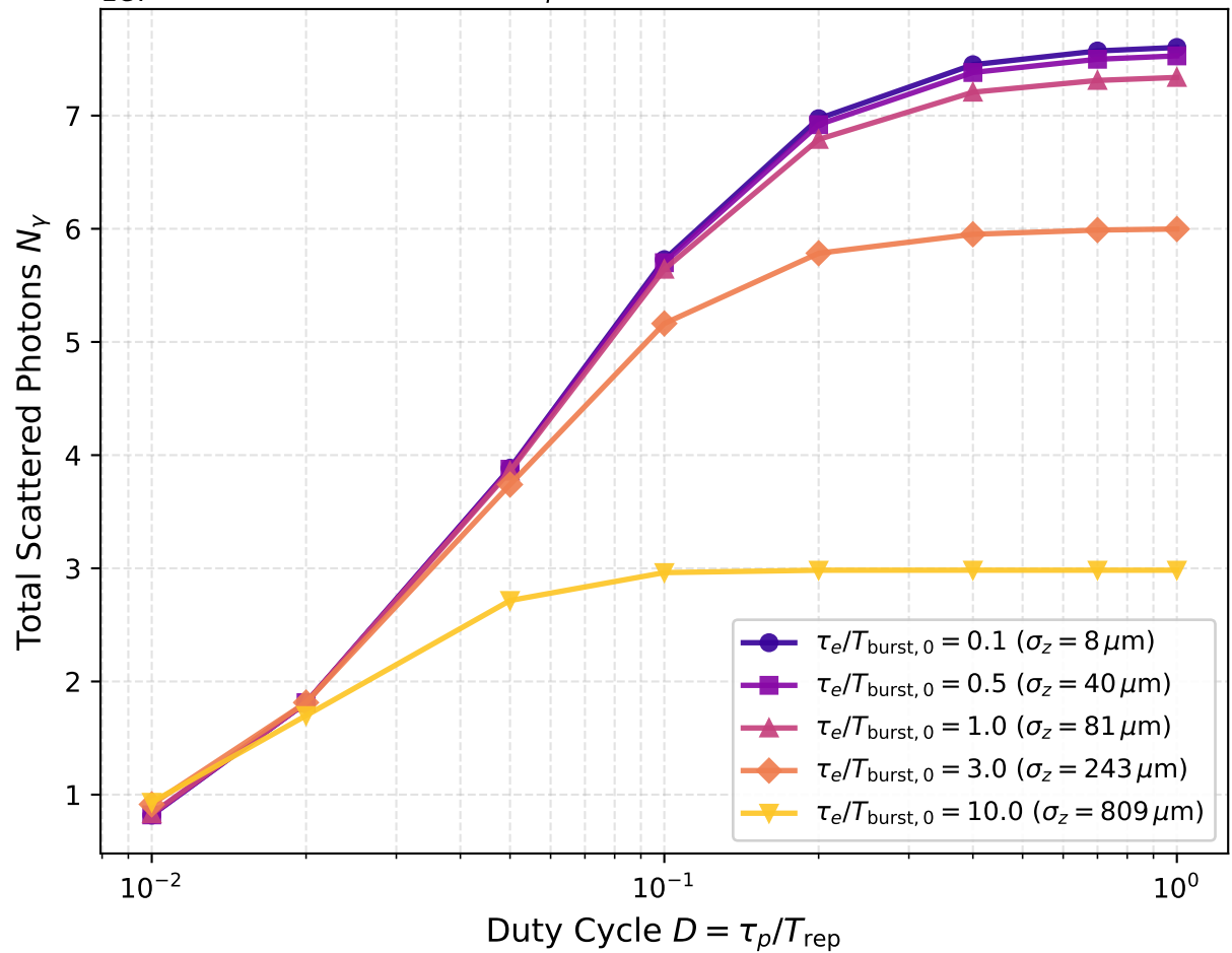
Absolute Yield ( N_p = 10 , E_{\text{tot}} = 1.0 \text{ J} , z_R = 3534 \mu\text{m} )
