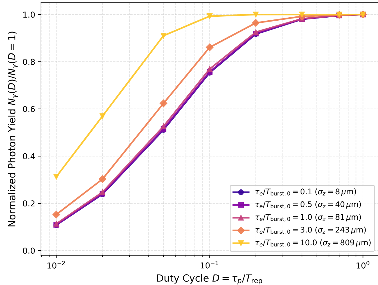
Relative Yield Retention vs. Duty Cycle
