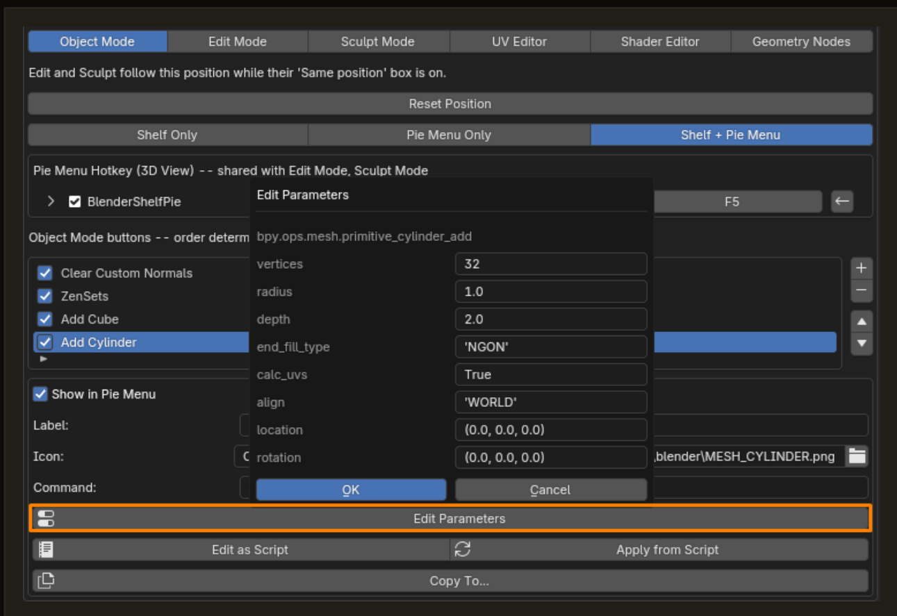
Edit Parameters: tweaking a cylinder's parameters without Python
