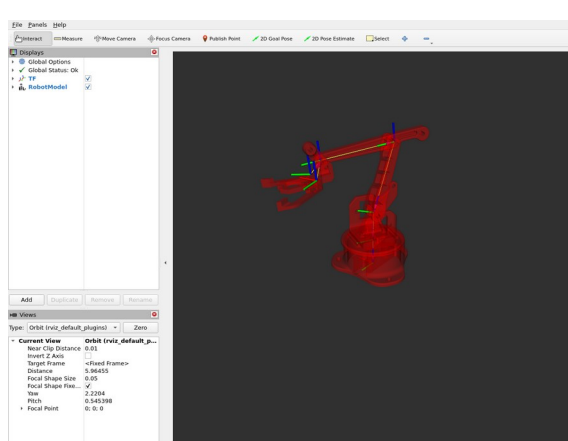
Figure 9. Preparation run: RViz started 8 s after robot_state_publisher; joint 1 = -0.5, joint 2 = 0.3, joint 3 = -0.4, joint 4 = -0.6 (gripper open). Genuine screenshot of the delivered workspace (category C), 28 Sep. 2026.
