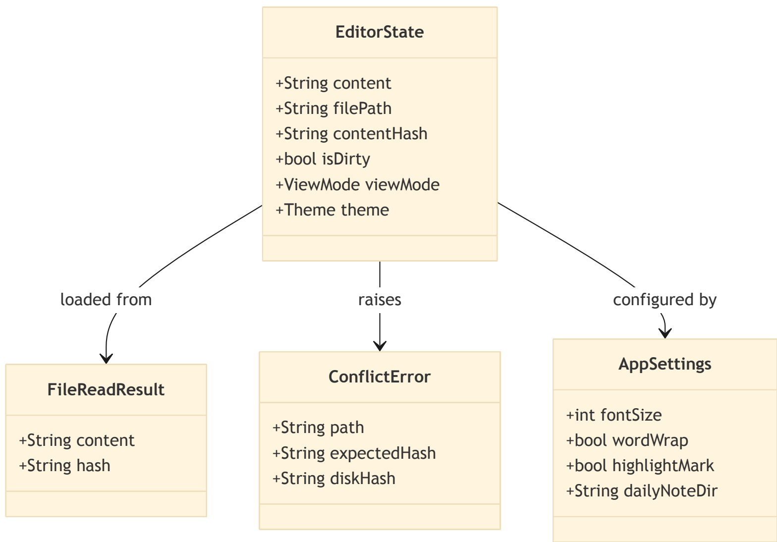
Class Diagram — Core Data Model
