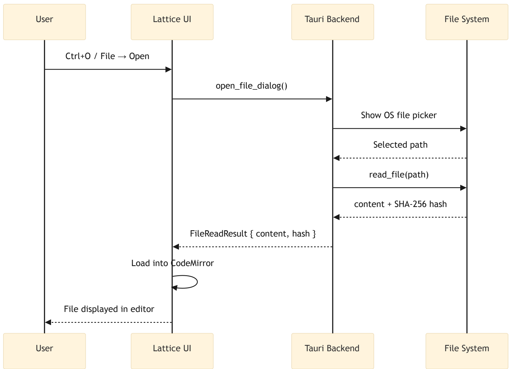
Sequence Diagram — File Open Flow
