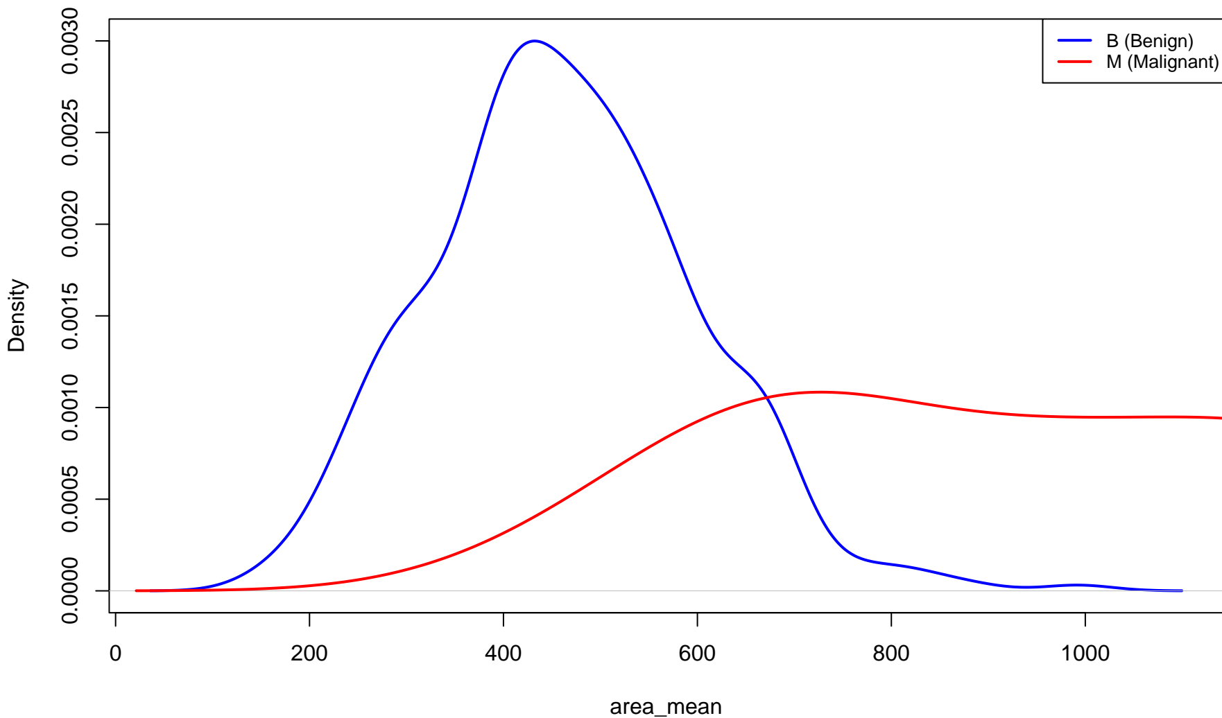
Density Plot: area_mean (B vs M)
