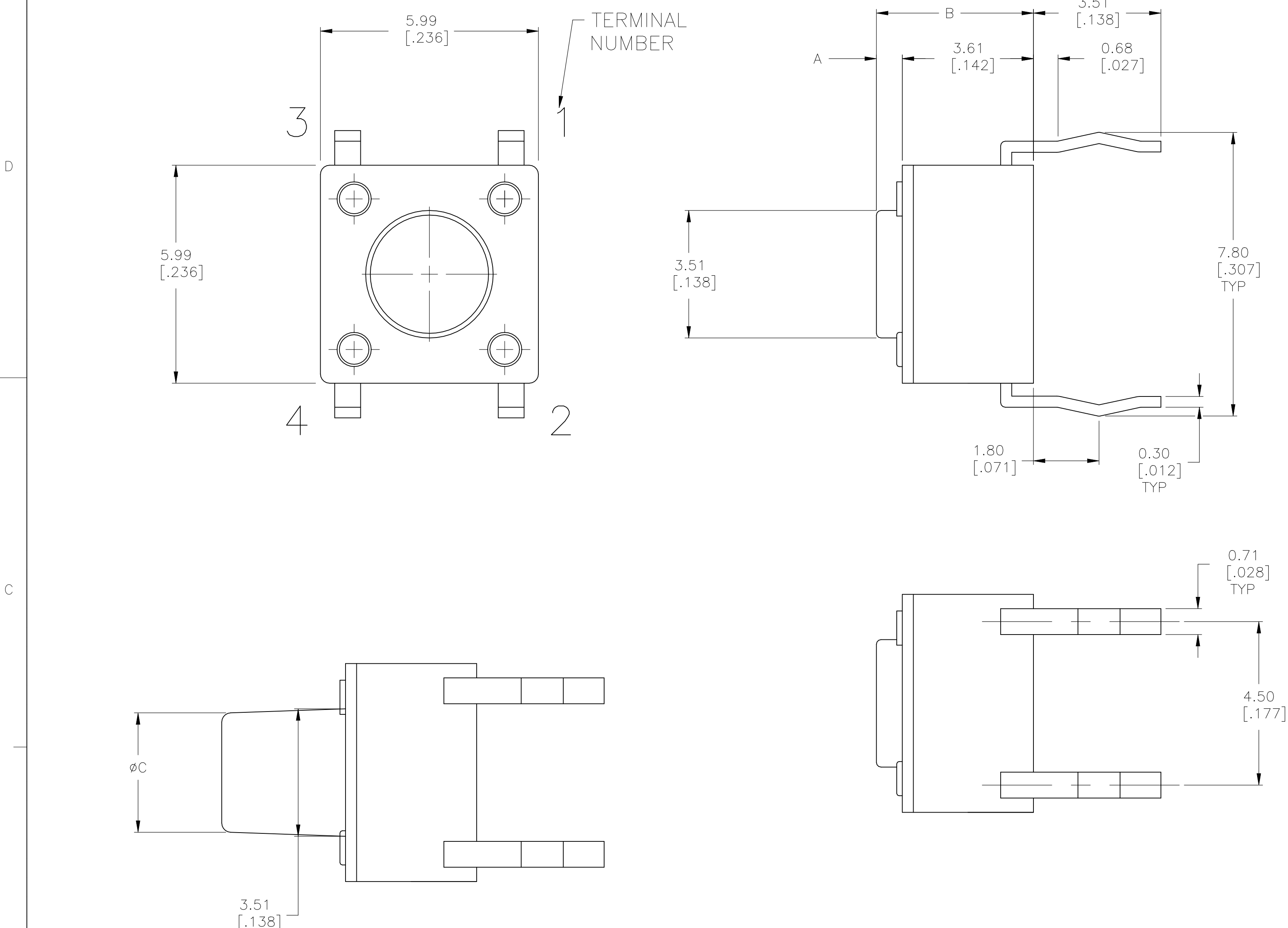
VIEW A-A FSM6J THRU FSM18J
