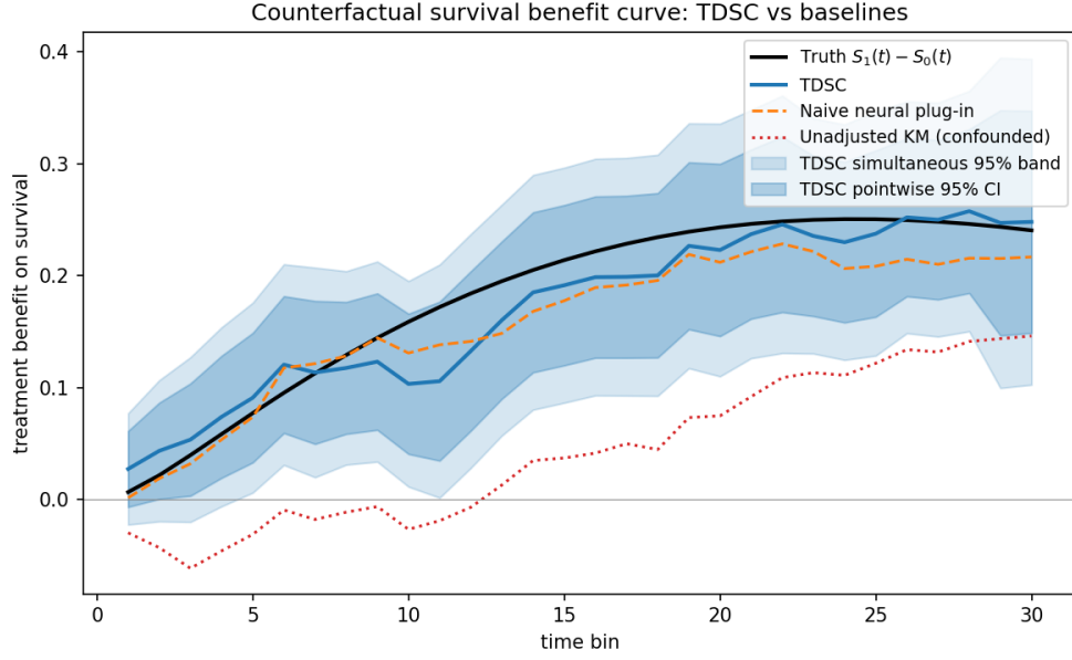
Figure 4: One replication ( n = 1000 , seed 7), shown for illustration. The TDSC benefit curve tracks the truth, which lies inside both the pointwise CI and the simultaneous band; the naive plug-in drifts low at later times, and unadjusted KM is severely biased (wrong-signed at early times).
