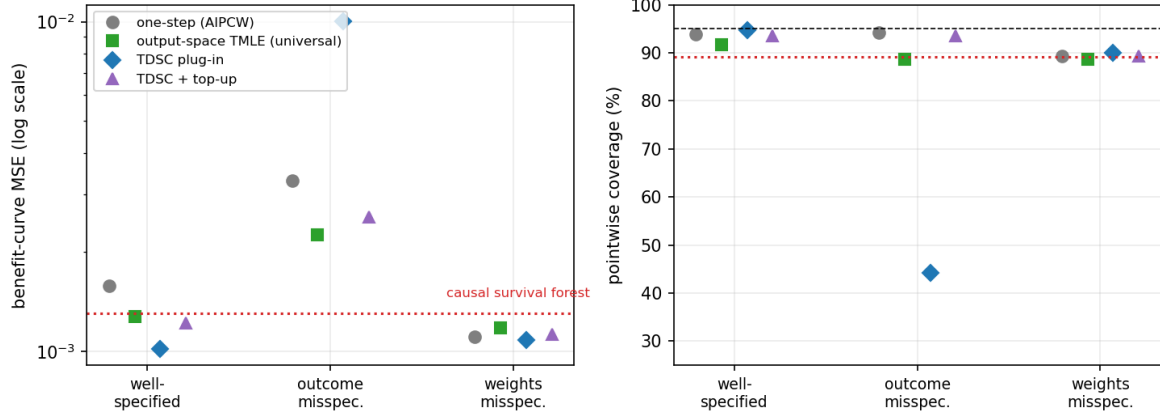
Figure 3: Head-to-head comparison across nuisance scenarios (benefit-curve MSE, log scale; pointwise coverage, 95% dashed): one-step, universal output-space TMLE, TDSC plug-in, and TDSC top-up on identical nuisances, with the causal survival forest (own nuisances, horizons 5–25) as the dotted reference. Well-specified, the estimators order one-step \rightarrow output-space TMLE \rightarrow TDSC; under outcome misspecification the plug-in is the most exposed—it estimates the working parameter—while the top-up and one-step remain nominal.
