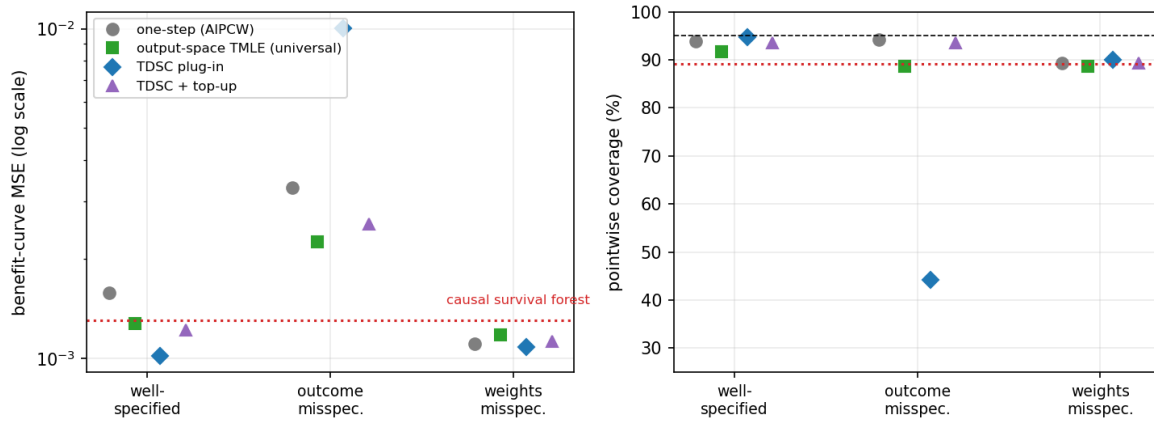
Figure 3: Head-to-head comparison across nuisance scenarios (benefit-curve MSE, log scale; pointwise coverage, 95% dashed): one-step, universal output-space TMLE, TDSC plug-in, and TDSC top-up on identical nuisances, with the causal survival forest (own nuisances, horizons 5–25) as the dotted reference. Well-specified, the estimators order one-step \rightarrow output-space TMLE \rightarrow TDSC; under outcome misspecification the plug-in is the most exposed—it estimates the working parameter—while the top-up and one-step remain nominal.
