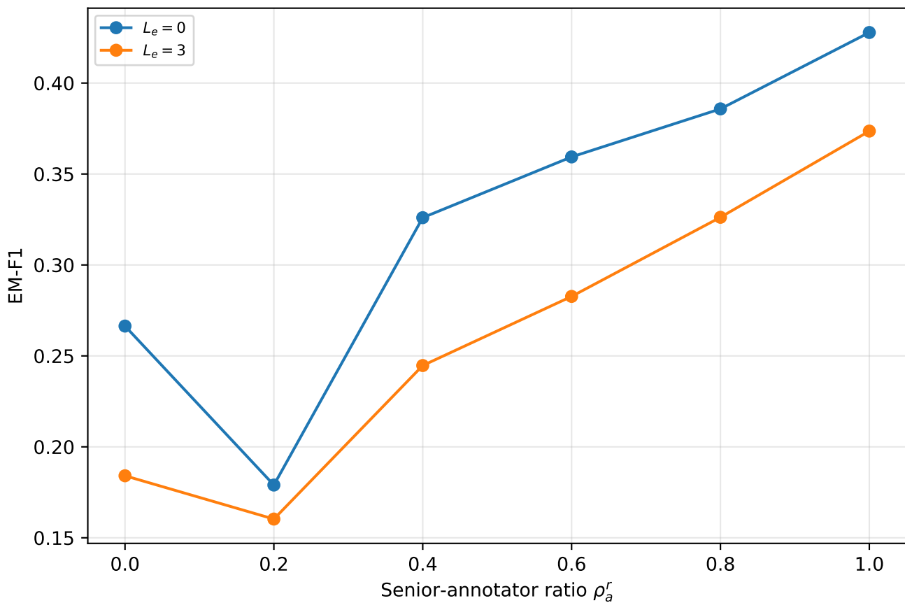
F1 vs annotation quality (training at L_t = 3 ) — EN
