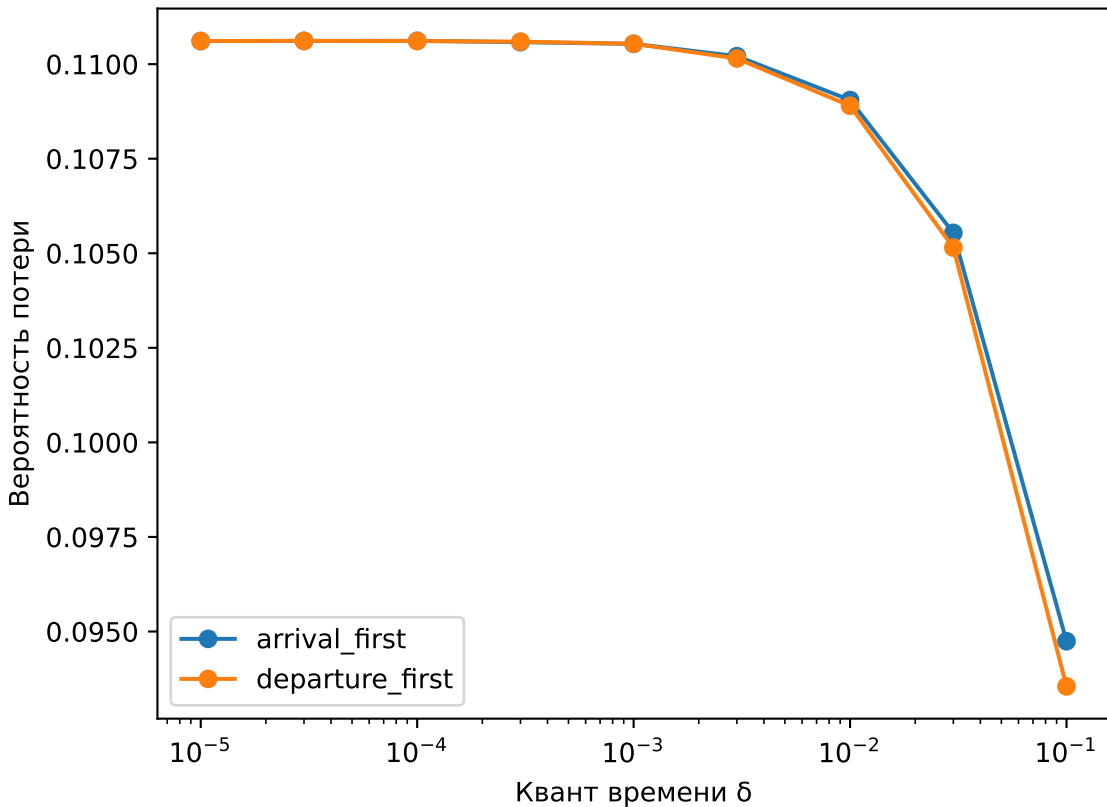
Packet loss, \rho=1.0 , K=8
