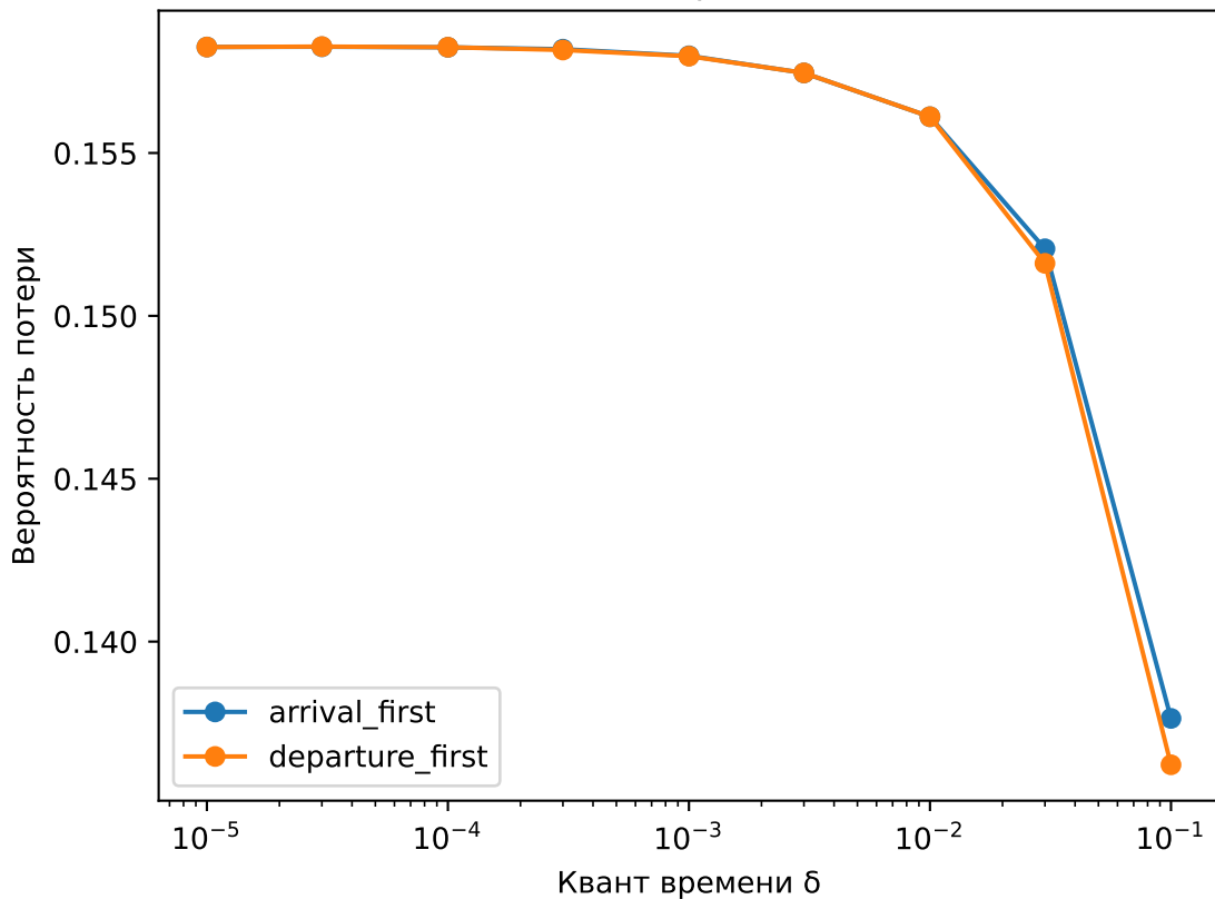
Packet loss, \rho=1.1 , K=8
