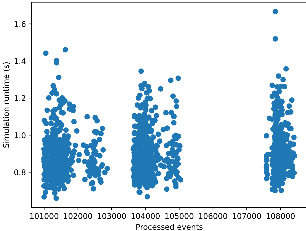
Runtime versus processed events
