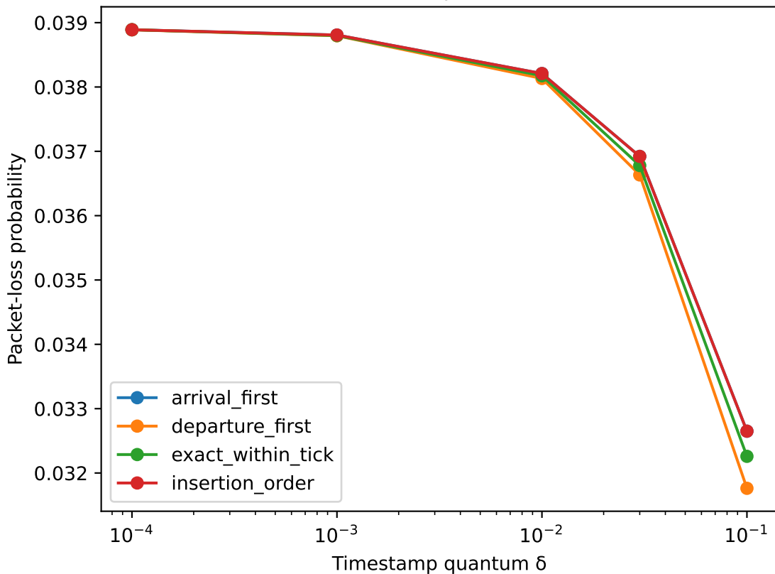
Packet loss, \rho=0.8 , K=8
