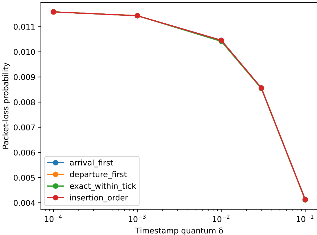
Packet loss, \rho=0.95 , K=32
