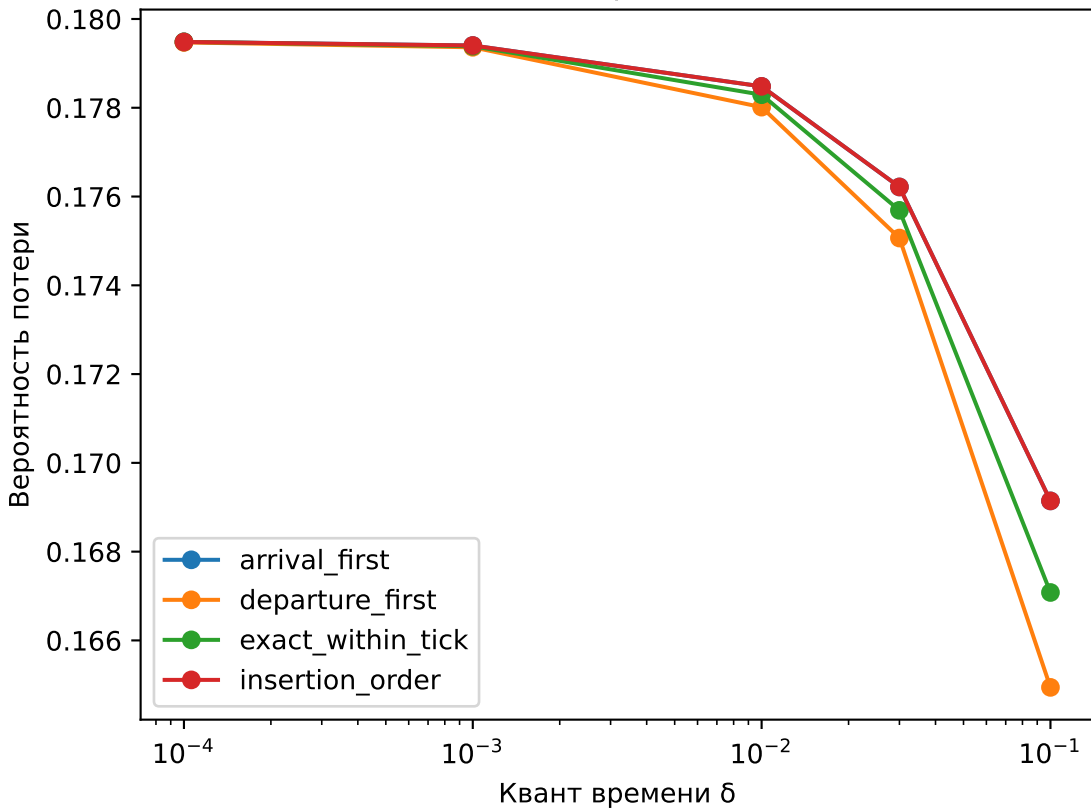
Packet loss, \rho=0.95 , K=4
