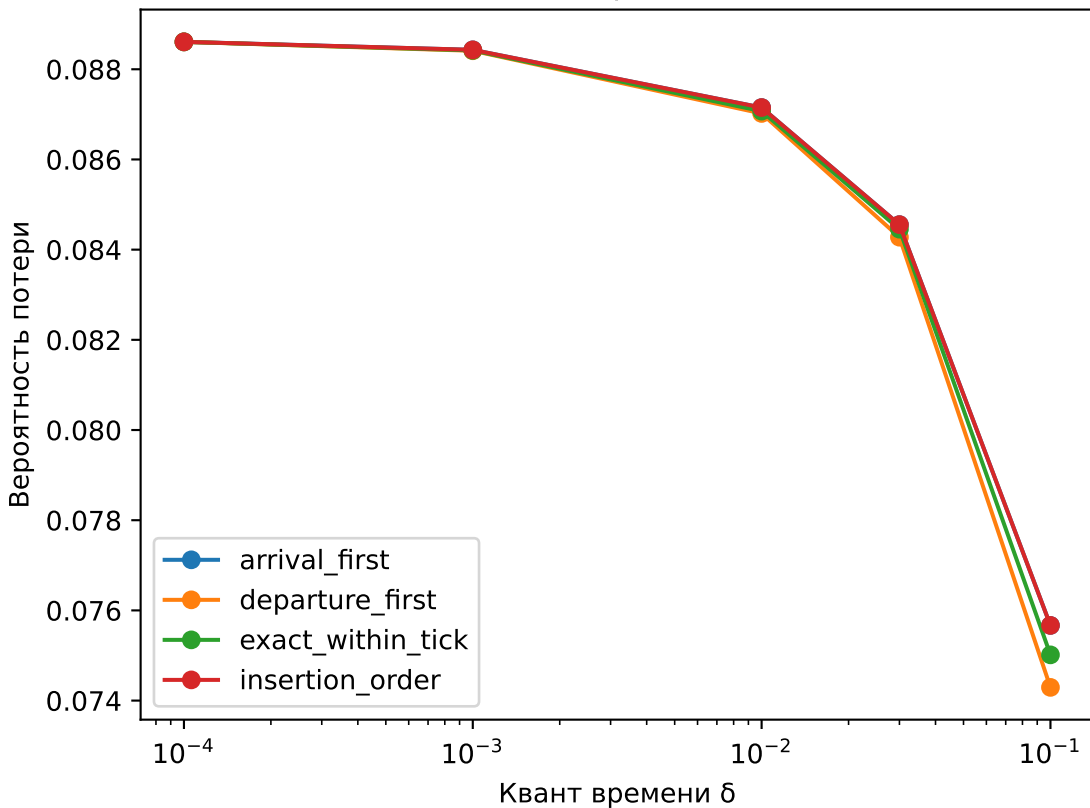
Packet loss, \rho=0.95 , K=8
