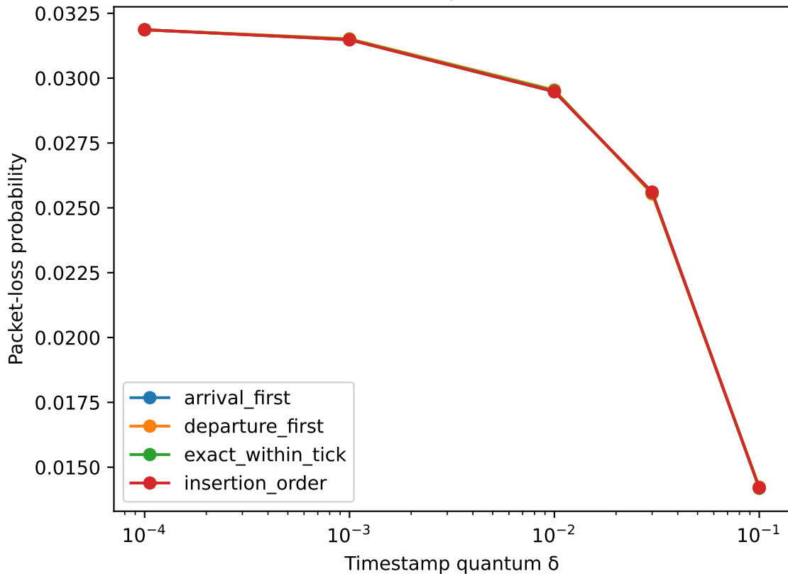
Packet loss, \rho=1.0 , K=32
