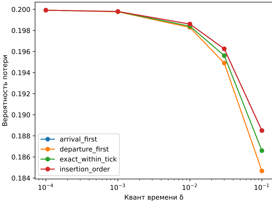
Packet loss, \rho=1.0 , K=4
