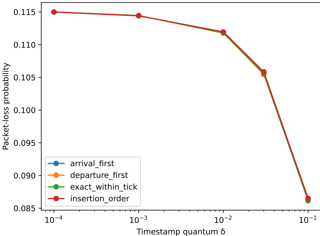
Packet loss, \rho=1.1 , K=16
