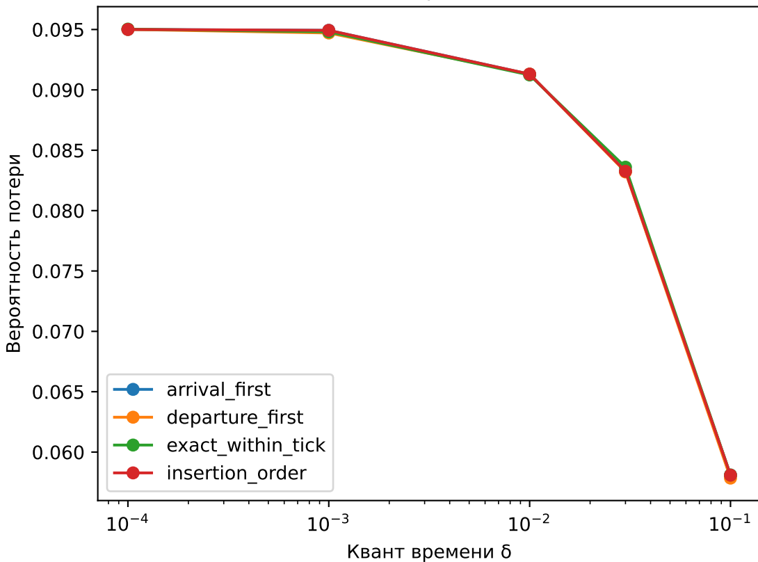
Packet loss, \rho=1.1 , K=32
