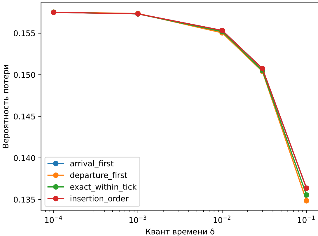
Packet loss, \rho=1.1 , K=8
