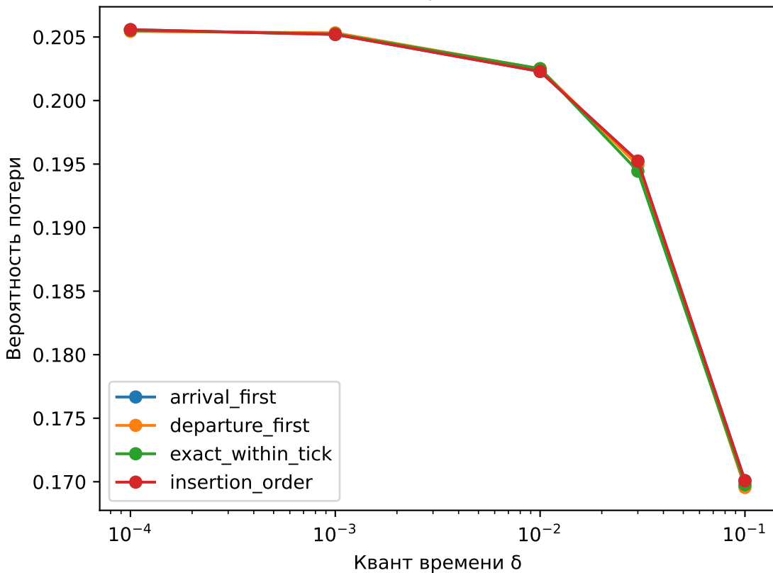
Packet loss, \rho=1.25 , K=16
