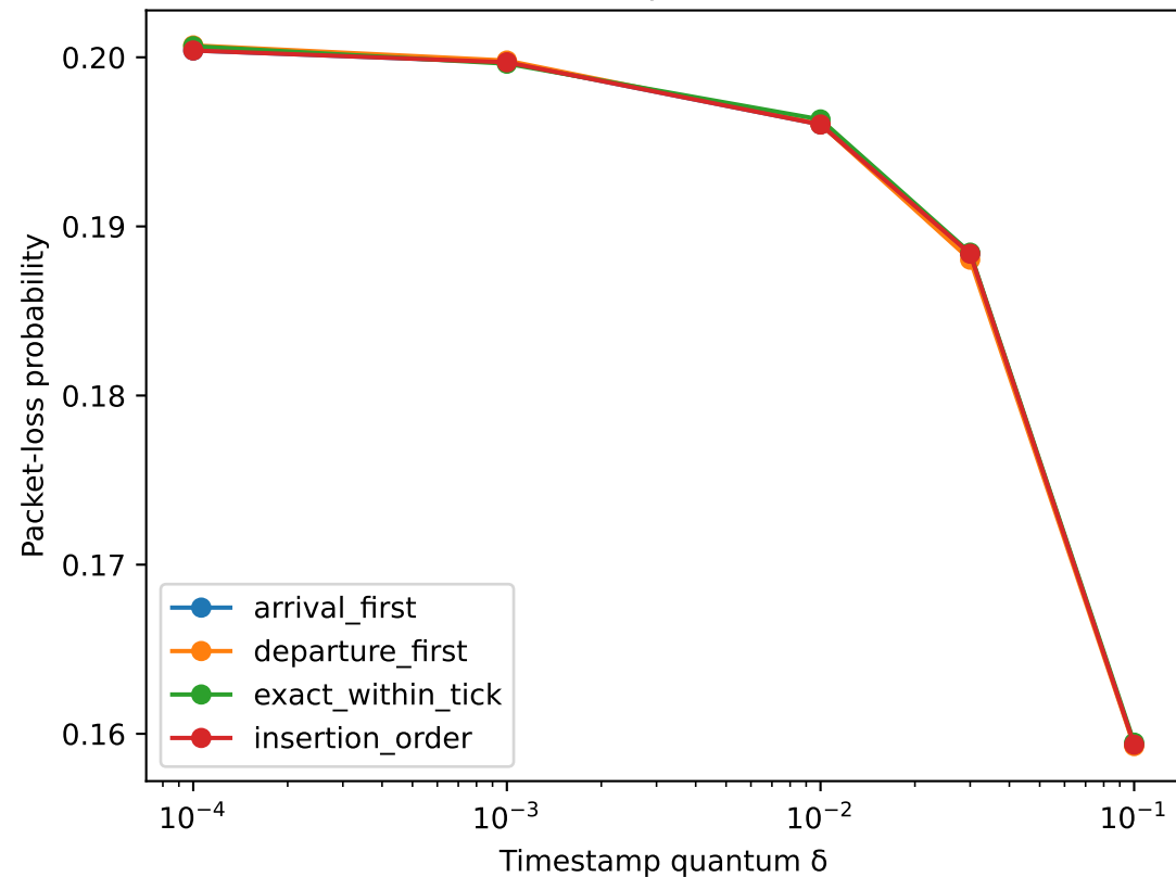
Packet loss, \rho=1.25 , K=32
