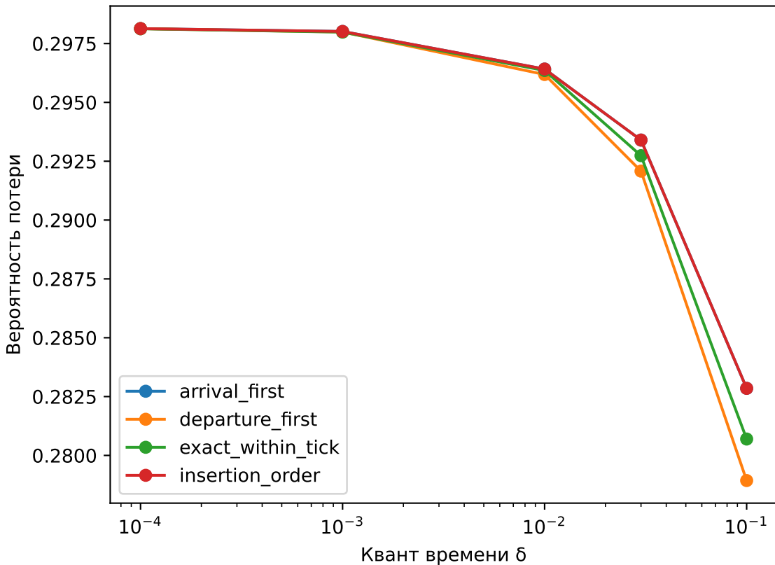
Packet loss, \rho=1.25 , K=4
