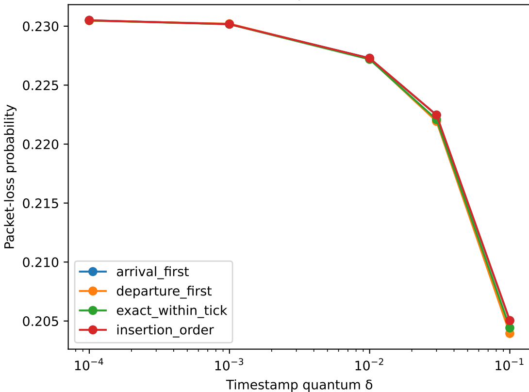
Packet loss, \rho=1.25 , K=8
