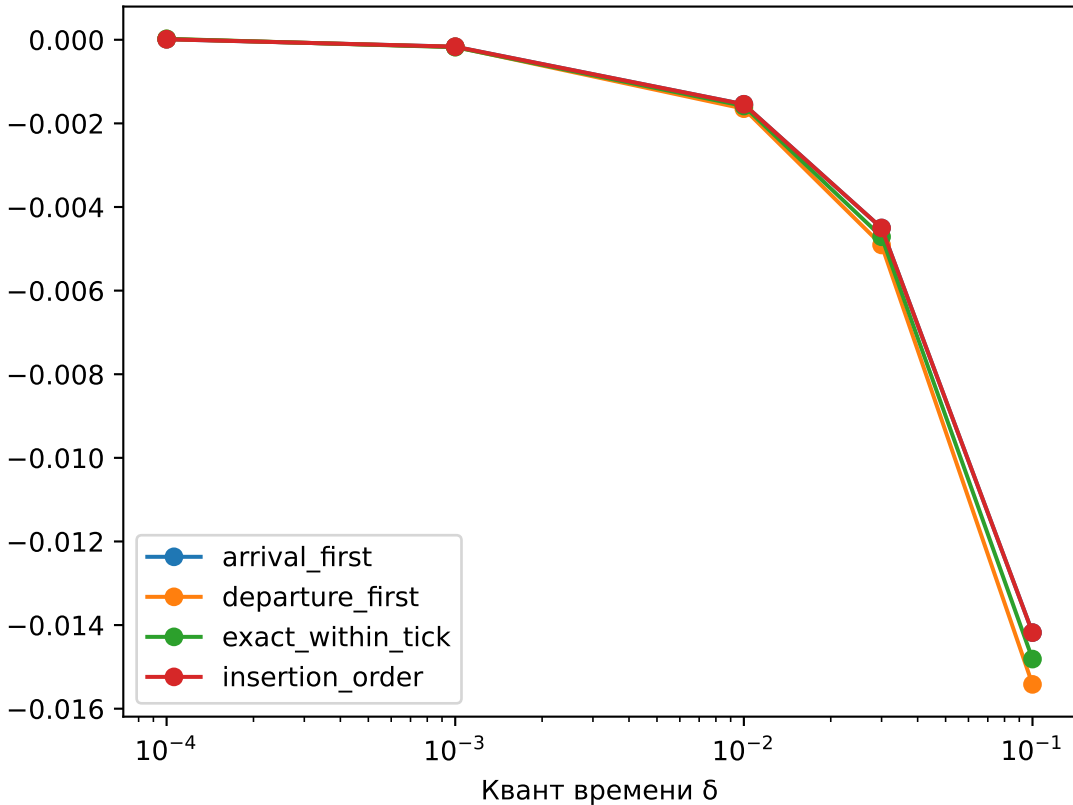
Signed Loss Error
