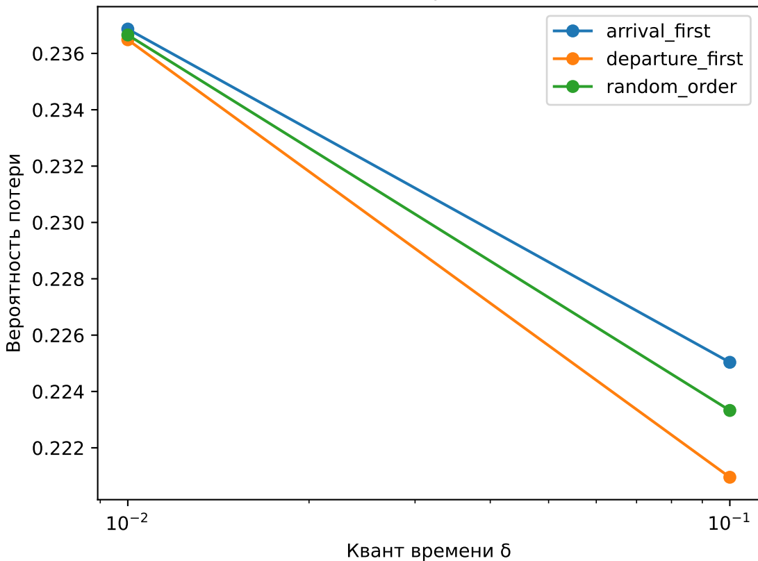
Packet loss, \rho=1.1 , K=4
