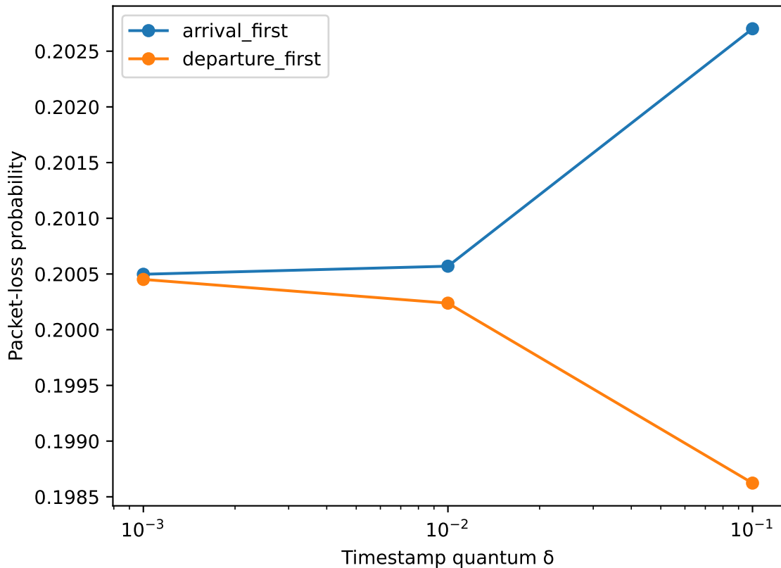
Packet loss, \rho=1.0 , K=4
