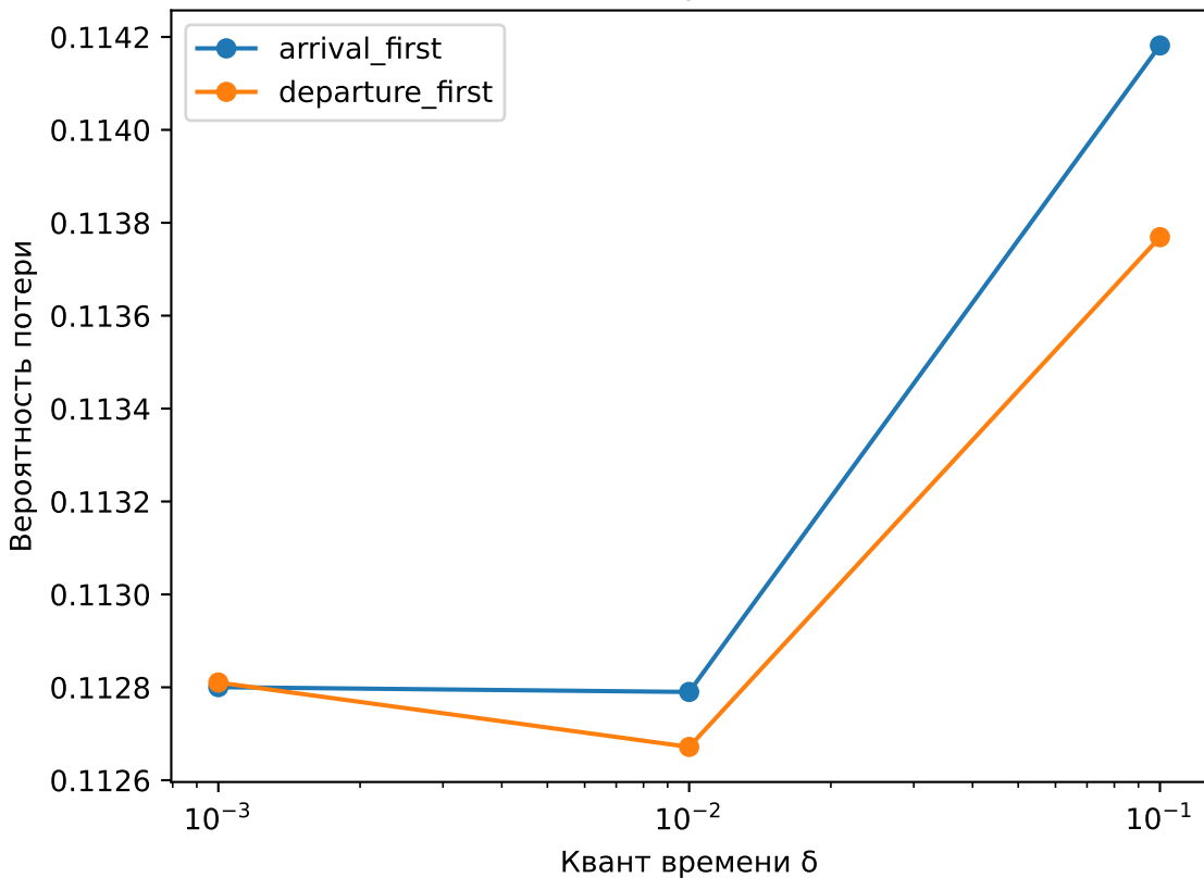
Packet loss, \rho=1.1 , K=16
