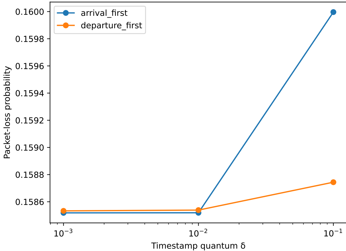
Packet loss, \rho=1.1 , K=8
