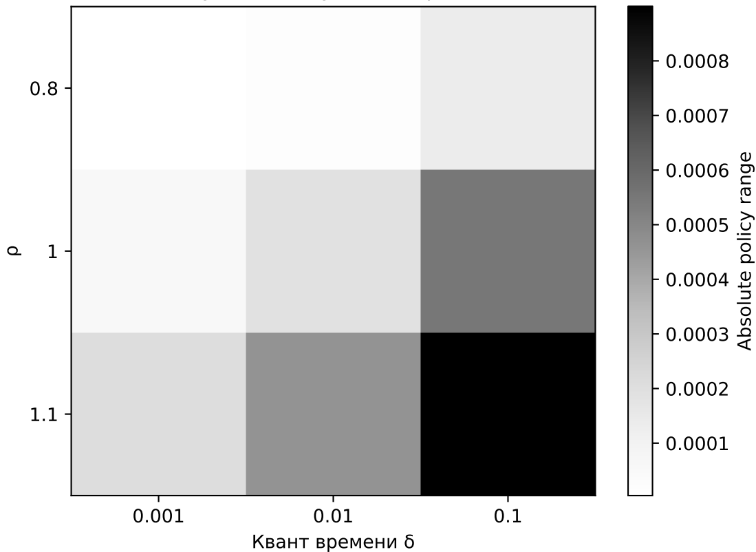
Policy sensitivity heatmap, K=16
