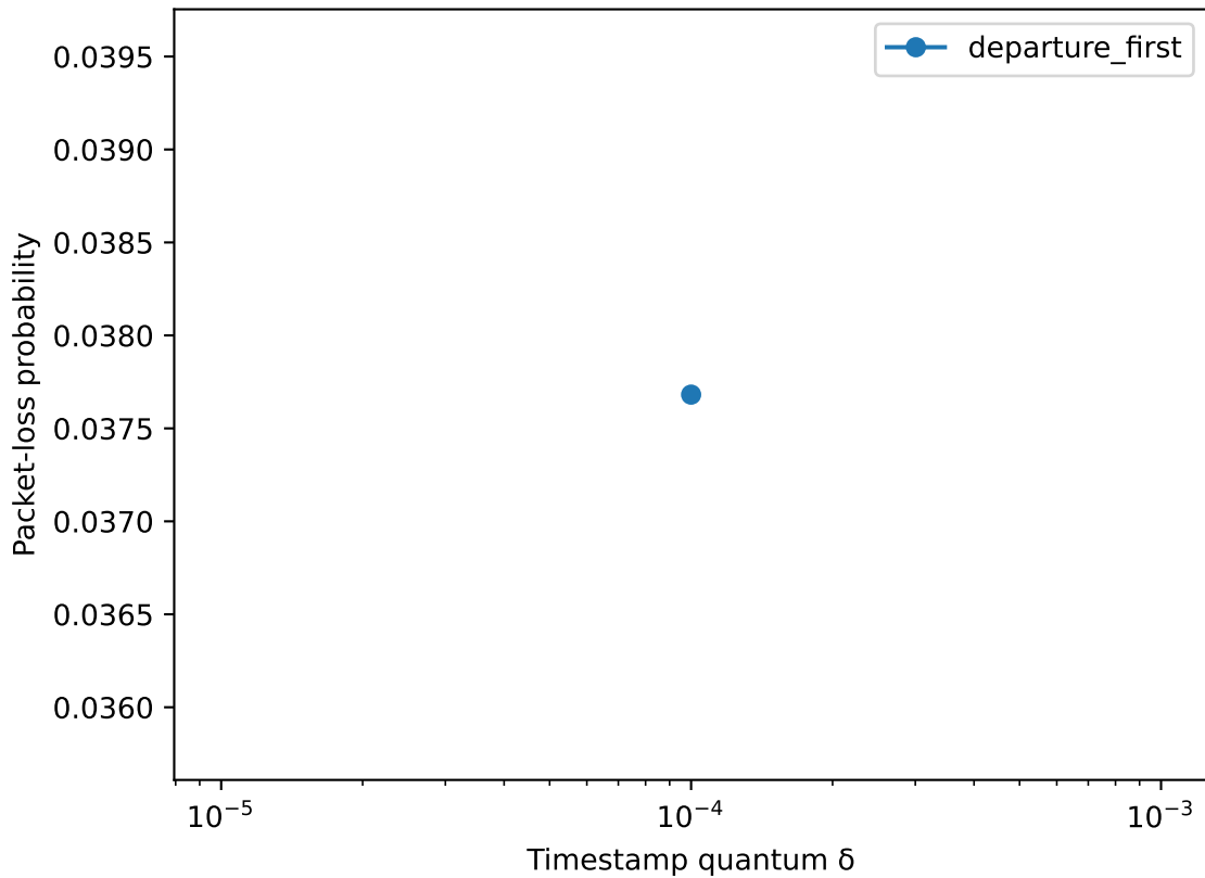
Packet loss, \rho=0.95 , K=16
