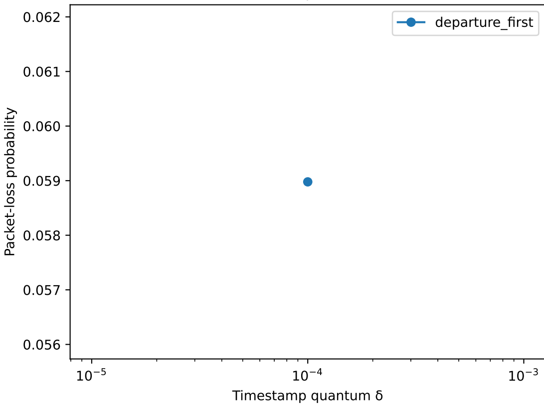
Packet loss, \rho=1.0 , K=16
