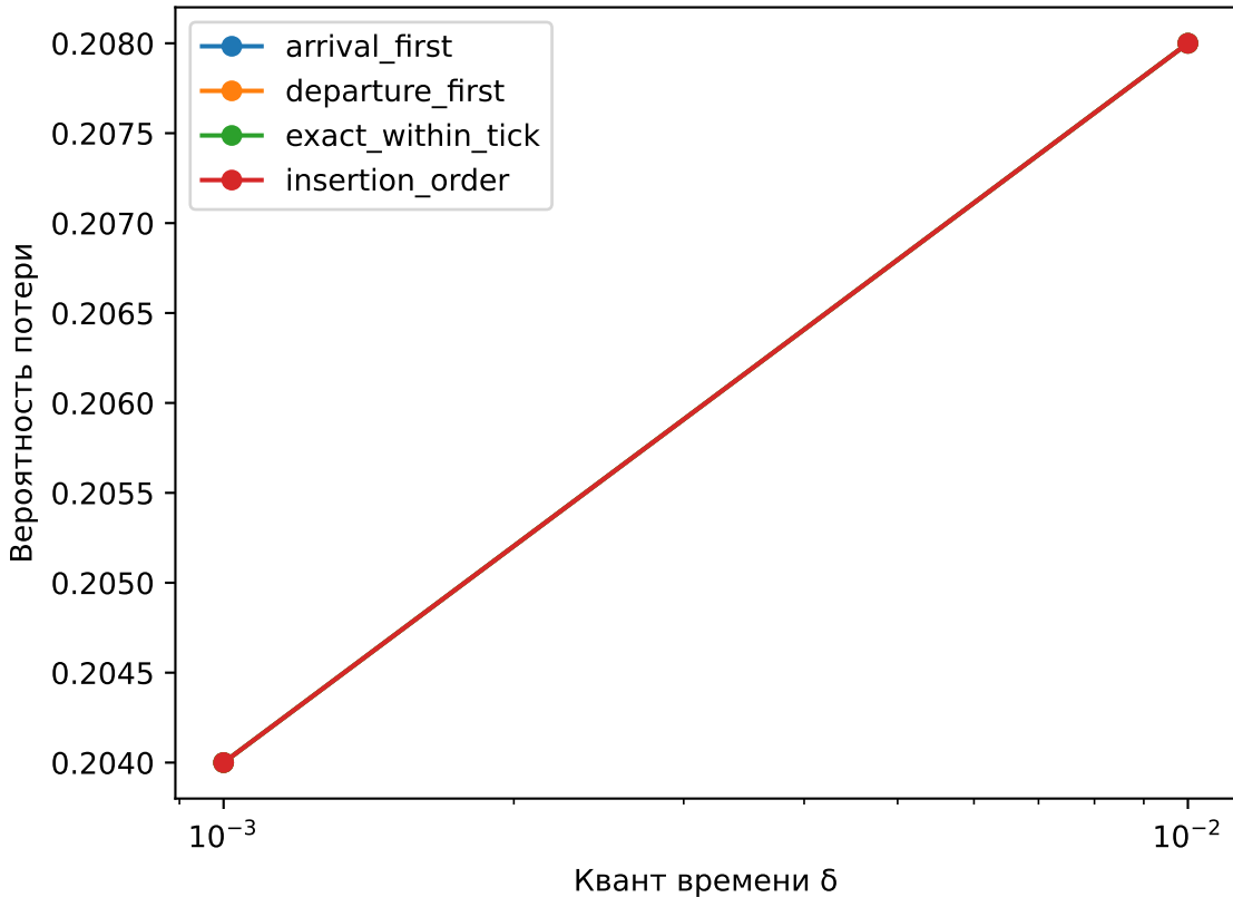
Packet loss, \rho=1.1 , K=4
