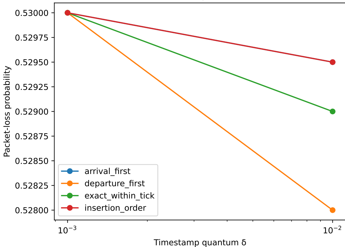
Packet loss, \rho=1.1 , K=1
